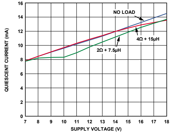
Figure 19. Quiescent Current vs. Supply Voltage, Mono Mode, No Load, R_L = 4\Omega + 15\mu H , R_L = 2\Omega + 7.5\mu H
