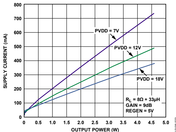
Figure 23. Supply Current vs. Output Power into 8\Omega ; PVDD = 7 V, PVDD = 12 V, PVDD = 18 V
