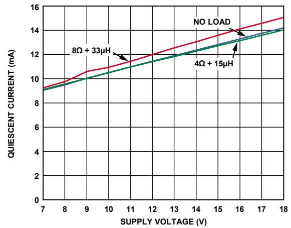
Figure 18. Quiescent Current vs. Supply Voltage, R_L = 8\Omega + 33\mu H , No Load, R_L = 4\Omega + 15\mu H
