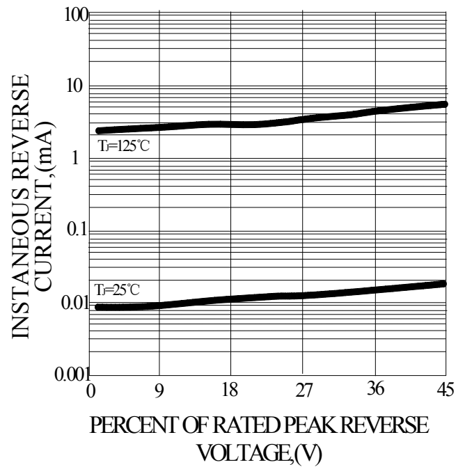
FIG.4-TYPICAL REVERSE CHARACTERISTICS
