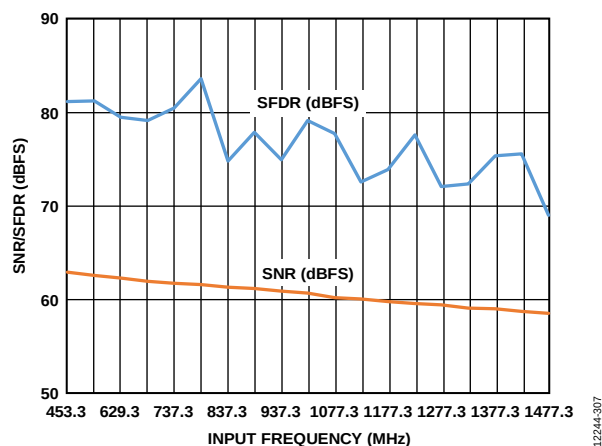
Figure 16. SNR/SFDR vs. Input Frequency; 450 \text{ MHz} < f_{IN} < 1500 \text{ MHz} ; Buffer Current = 7.5\times (Uses Circuit Shown in Figure 64)
