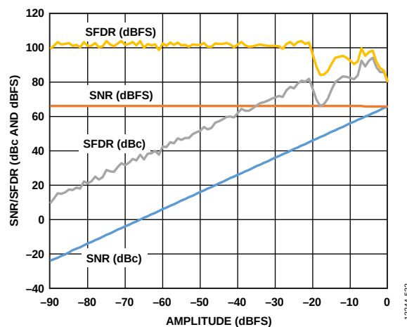
Figure 45. SNR/SFDR vs. Analog Input Level, f_{IN} = 10.3\text{ MHz} ; Buffer Current = 2.0x
