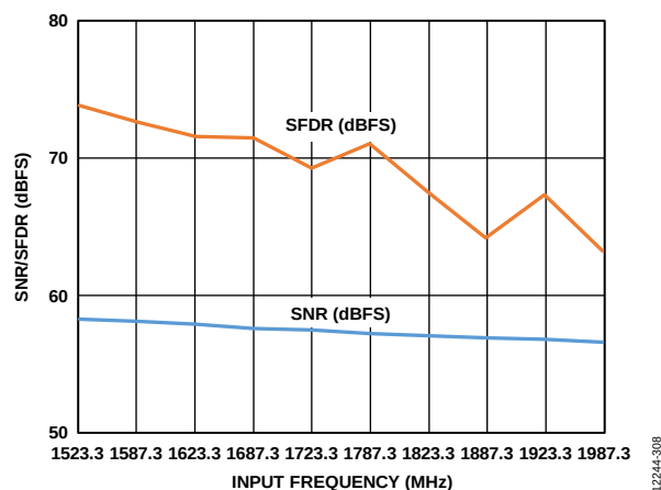
Figure 17. SNR/SFDR vs. Input Frequency; 1500 \text{ MHz} < f_{IN} < 2000 \text{ MHz} ; Buffer Current = 8.5\times (Uses Circuit Shown in Figure 64)
