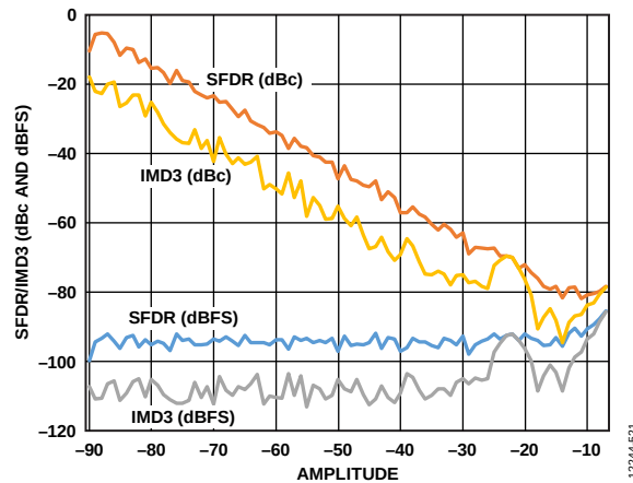
Figure 44. Two-Tone SFDR/IMD3 vs. Input Amplitude ( A_{IN} ) with f_{IN1} = 338\text{ MHz} and f_{IN2} = 341\text{ MHz}
