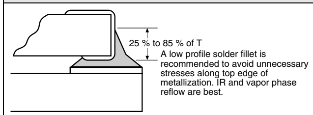
FIGURE 4 - RECOMMENDED MOUNTING 1)2)3)
