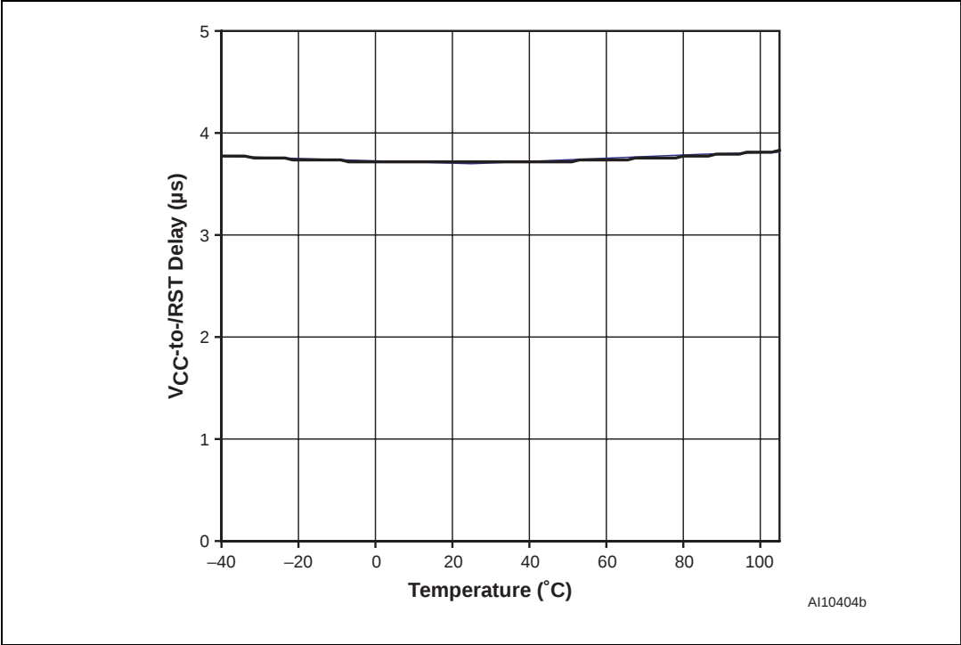
Figure 16. V_{CC} -to-reset output delay vs. temperature - V_{OD} = V_{TH} - V_{CC}
