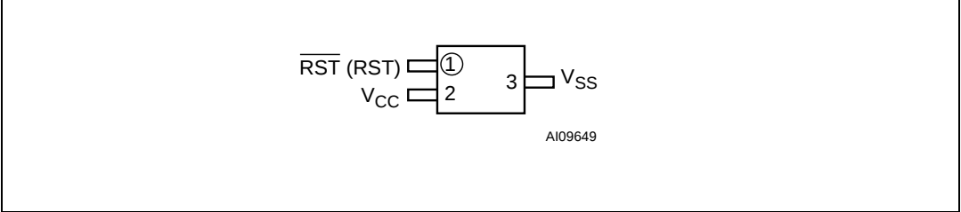
Figure 3. SOT23-3 connections
