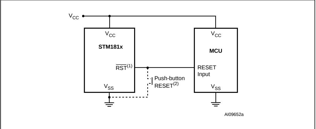
Figure 4. Hardware hookup
