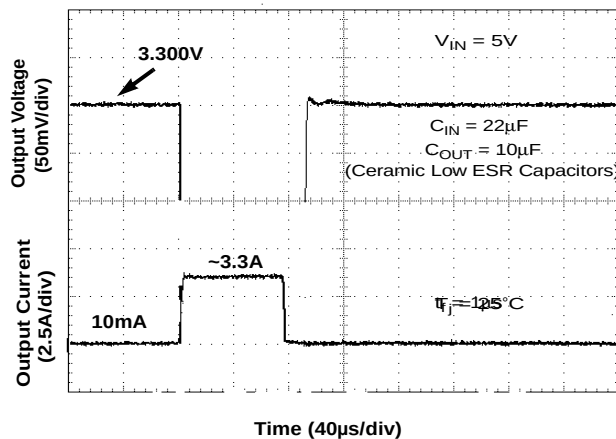
Short Circuit Removal Response
