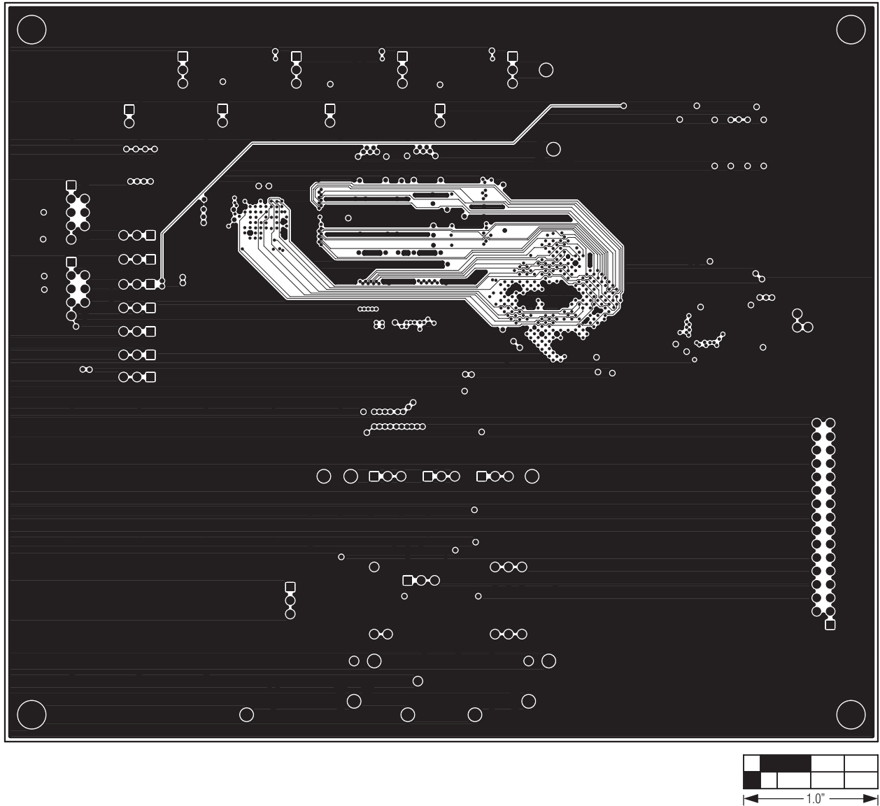
Figure 13. MAX11105 EV Kit PCB Layout—Layer 6
