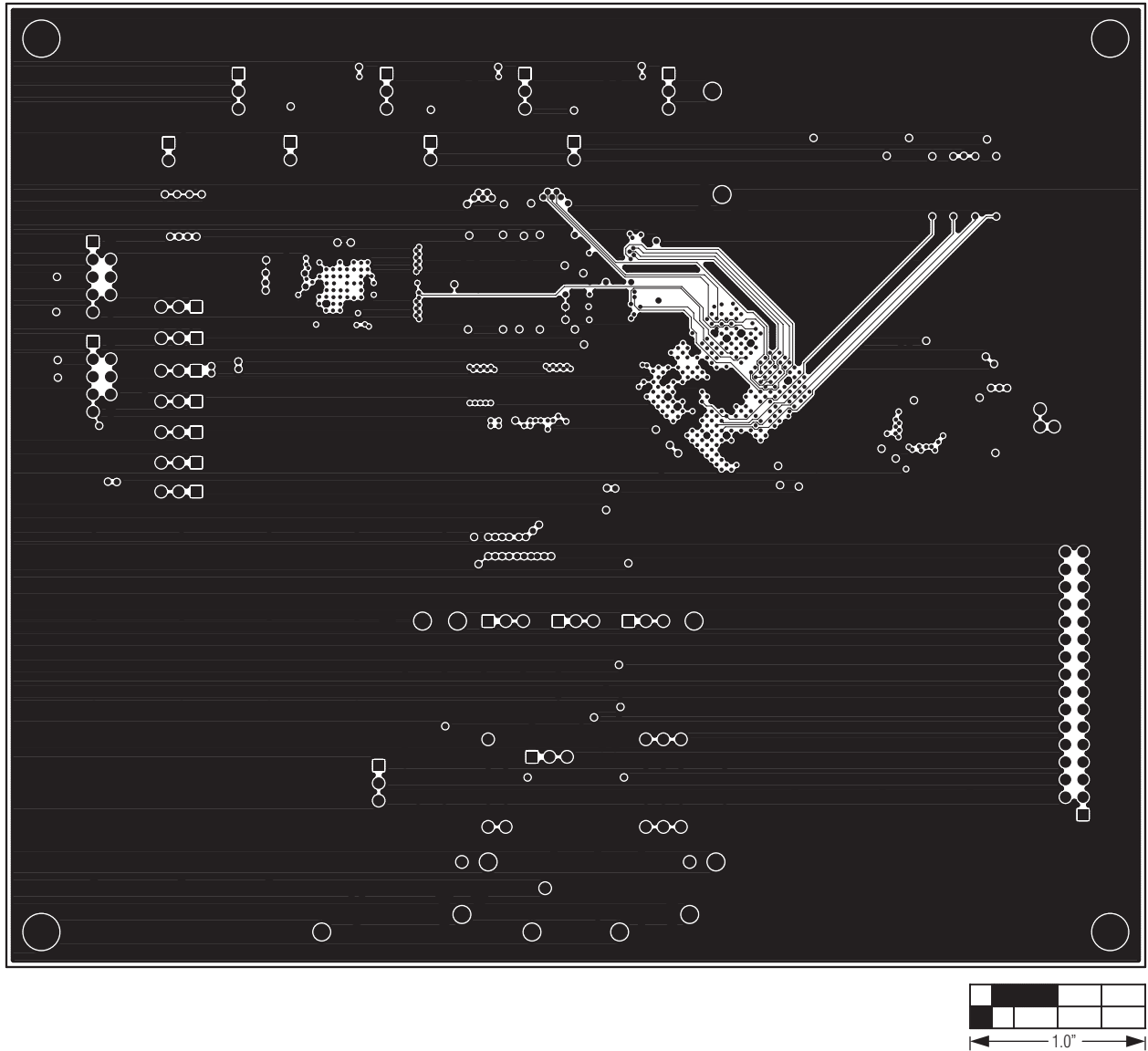
Figure 11. MAX11105 EV Kit PCB Layout—Layer 4
