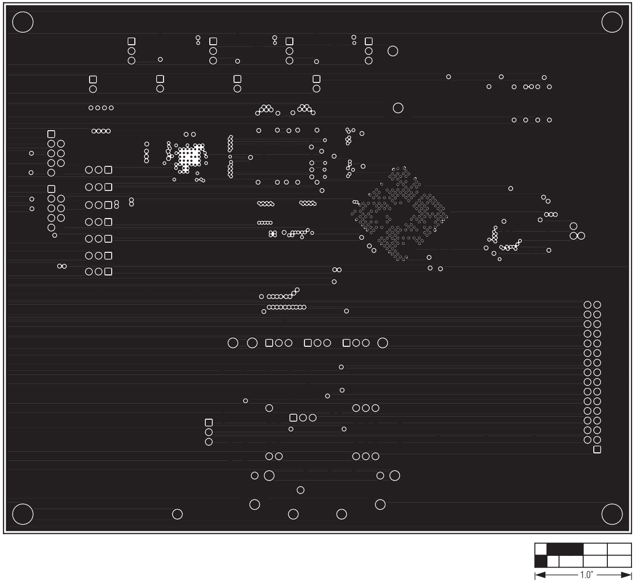
Figure 9. MAX11105 EV Kit PCB Layout—Layer 2
