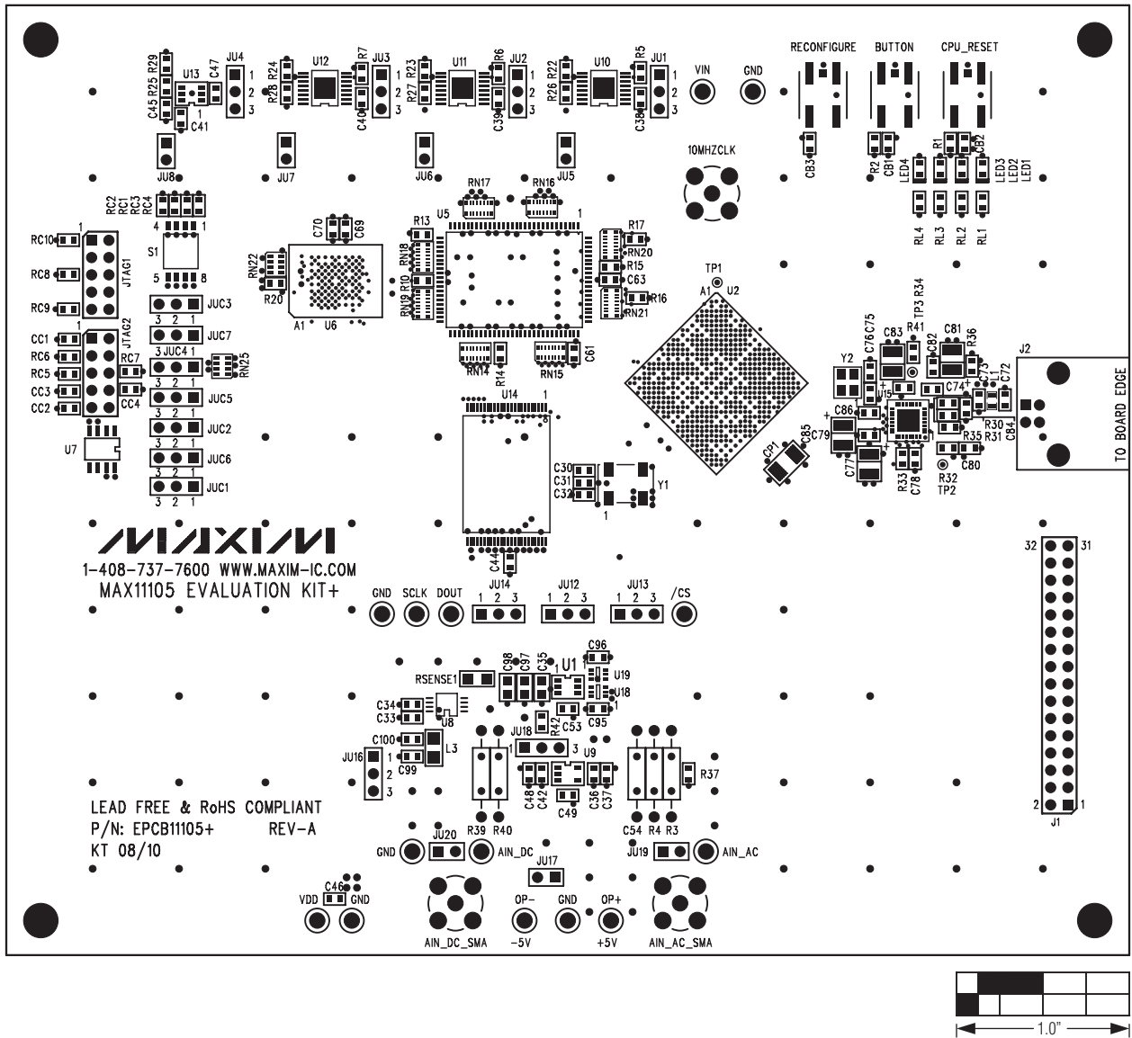
Figure 7. MAX11105 EV Kit Component Placement Guide—Top
