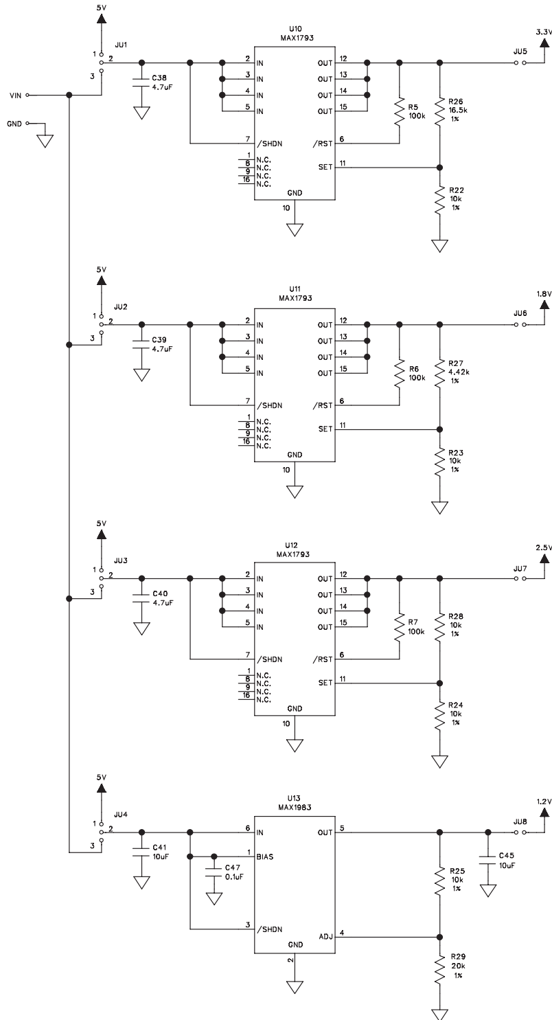
Figure 6k. MAX1105 EV Kit Schematic (Sheet 11 of 12)
