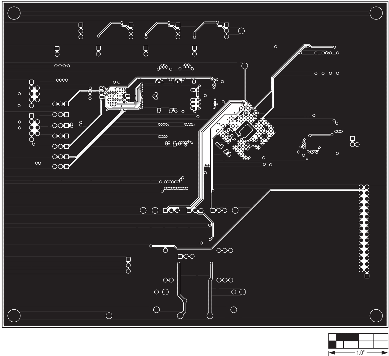
Figure 19. MAX11105 EV Kit PCB Layout—Bottom Side
