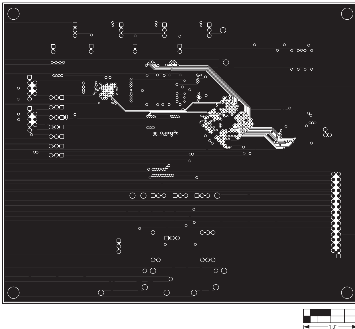
Figure 14. MAX11105 EV Kit PCB Layout—Layer 7
