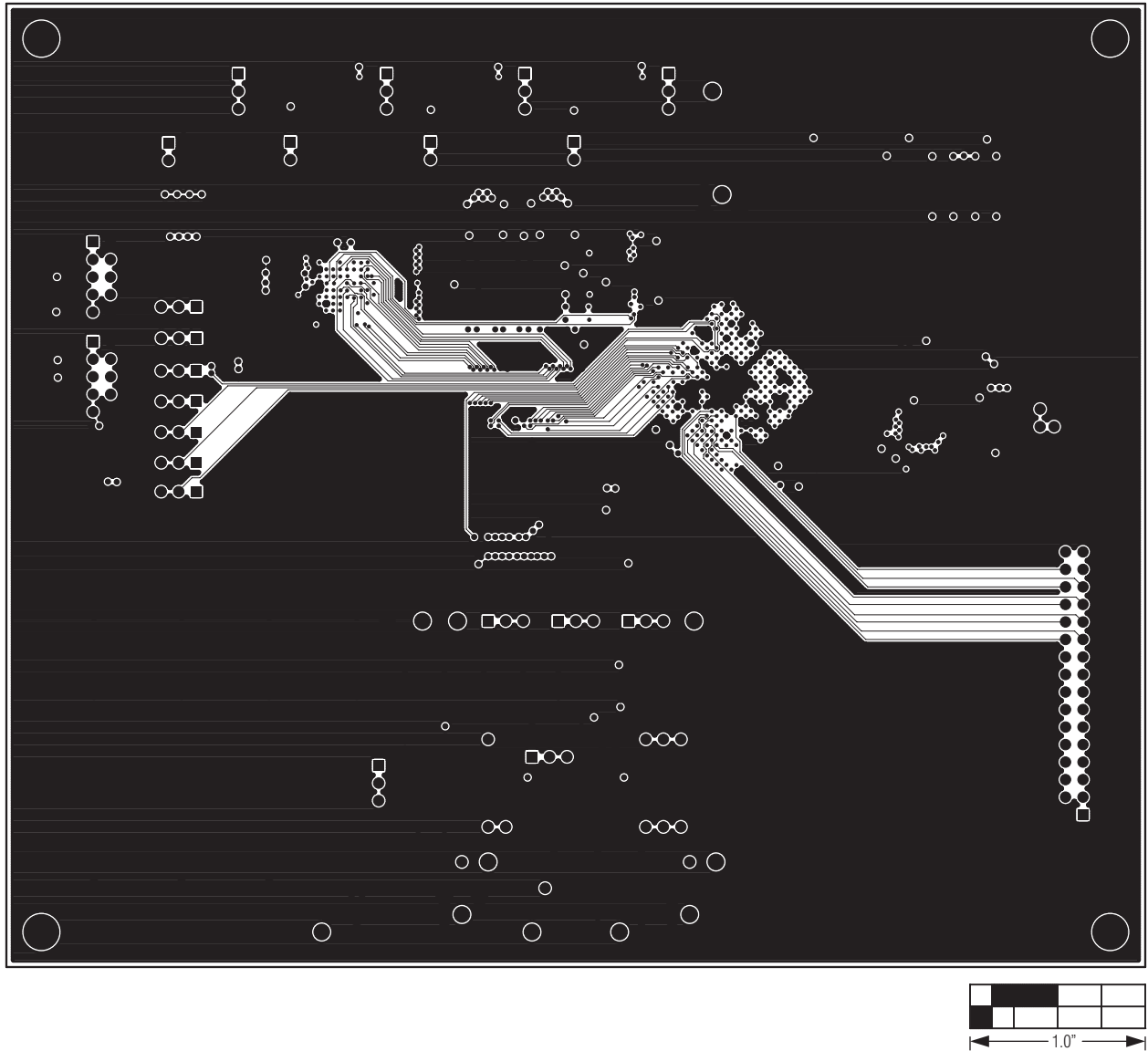
Figure 17. MAX11105 EV Kit PCB Layout—Layer 10
