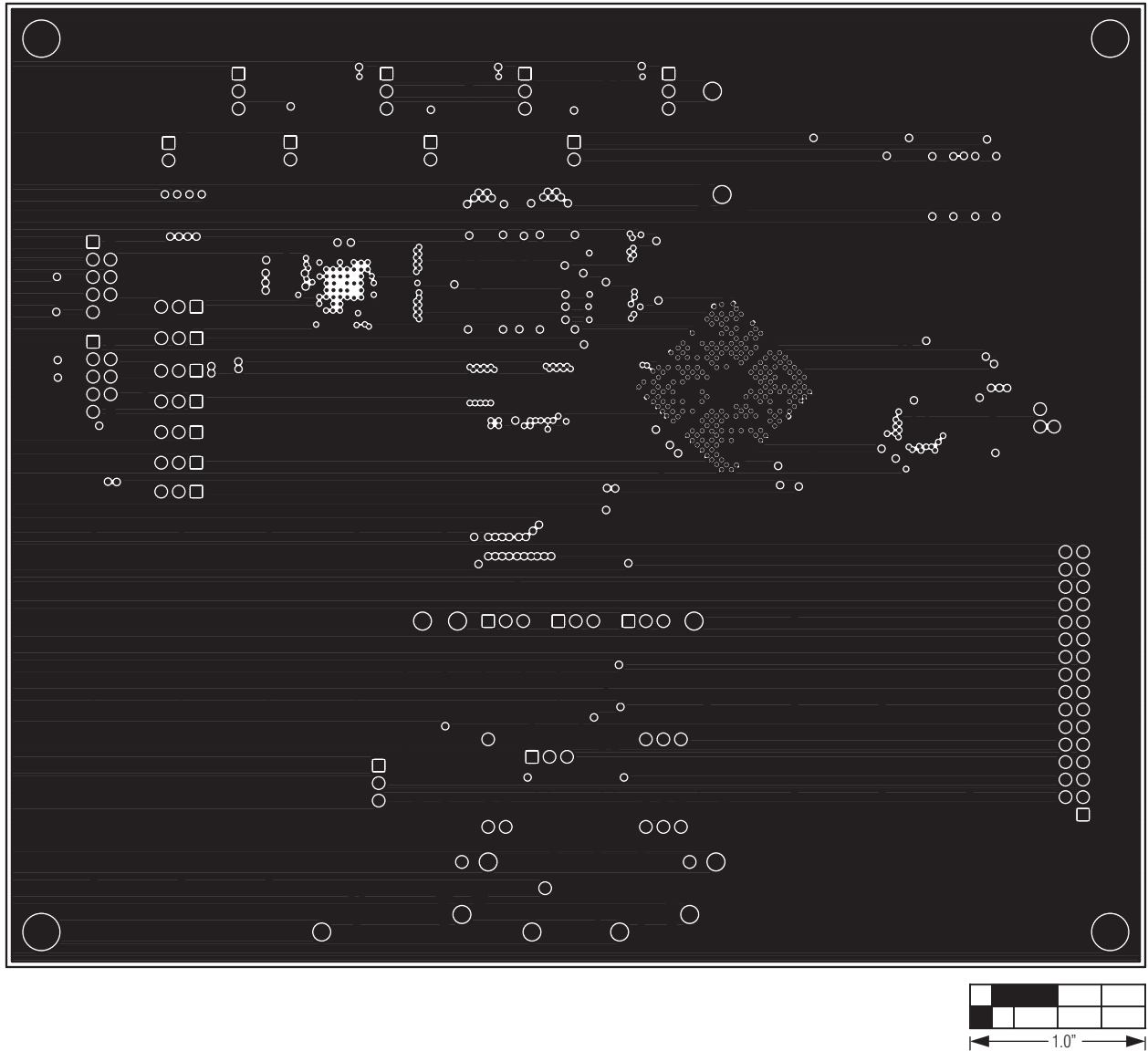
Figure 15. MAX11105 EV Kit PCB Layout—Layer 8
