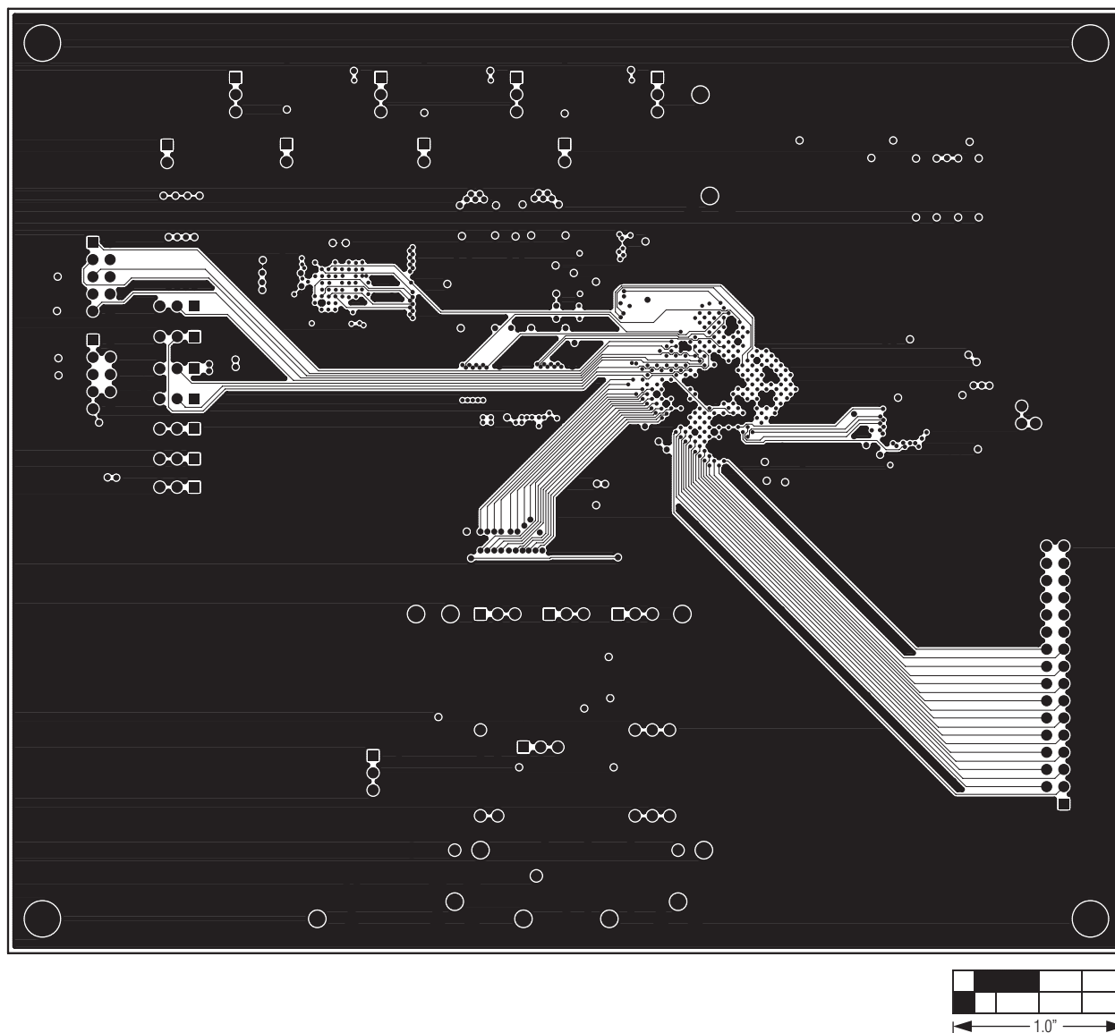
Figure 10. MAX11105 EV Kit PCB Layout—Layer 3
