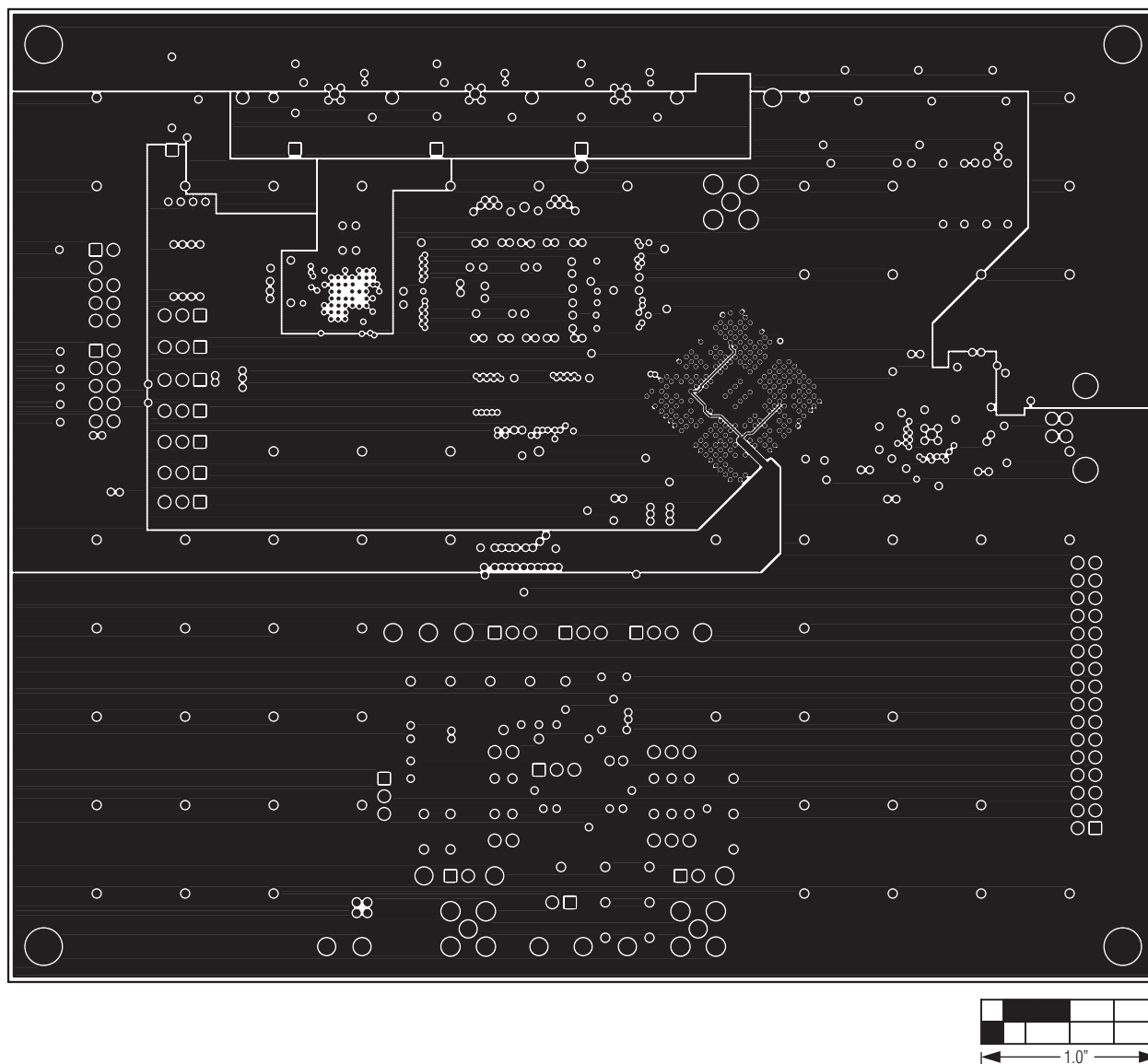
Figure 12. MAX11105 EV Kit PCB Layout—Layer 5
