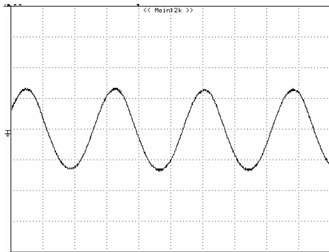
Figure 9: Input Terminal Ripple Current, i_c , at full rated output current and nominal input voltage with 12\mu\text{H} source impedance and 33\mu\text{F} electrolytic capacitor (100mV/div, 1us/div)
