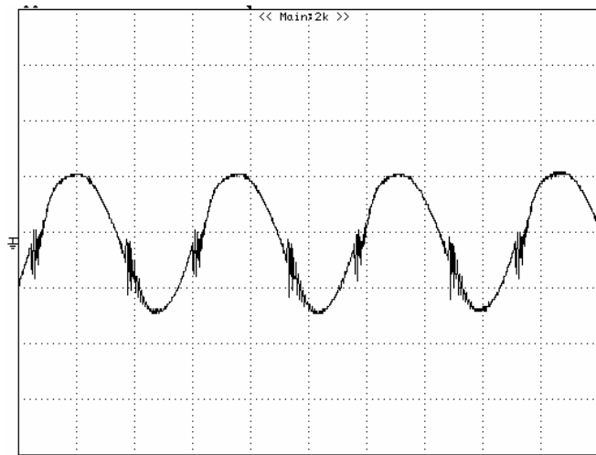
Figure 12: Output voltage ripple at nominal input voltage and rated load current ( I_o=5A ) (20mV/div, 1us/div) Load capacitance: 1μF ceramic capacitor and 10μF tantalum capacitor. Bandwidth: 20 MHz. Scope measurements should be made using a BNC cable (length shorter than 20 inches). Position the load between 51 mm to 76 mm (2 inches to 3 inches) from the module
