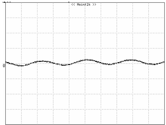
Figure 10: Input reflected ripple current, i_s , through a 12\mu\text{H} source inductor at nominal input voltage and rated load current (20mV/div, 1us/div)
