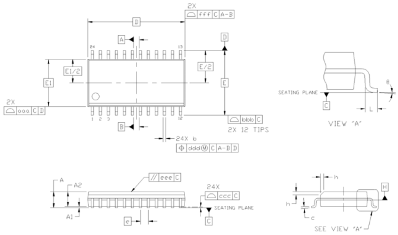
Figure 37. 24-Pin Wide Body SOIC
