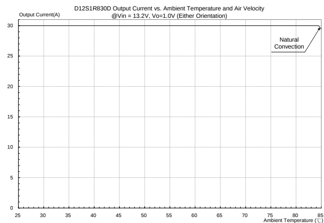
Figure 21: Output current vs. ambient temperature and air velocity@ V_{in}=13.2V , V_{out}=1.0V (Either Orientation)
