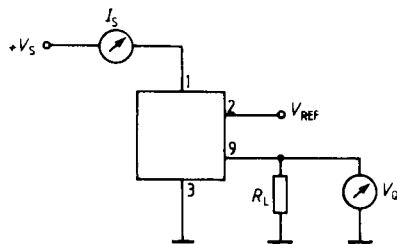
Test Circuit 1
