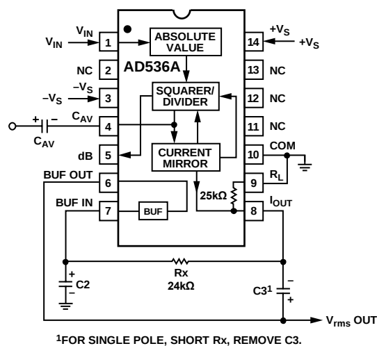
Figure 21. Two-Pole Postfilter
