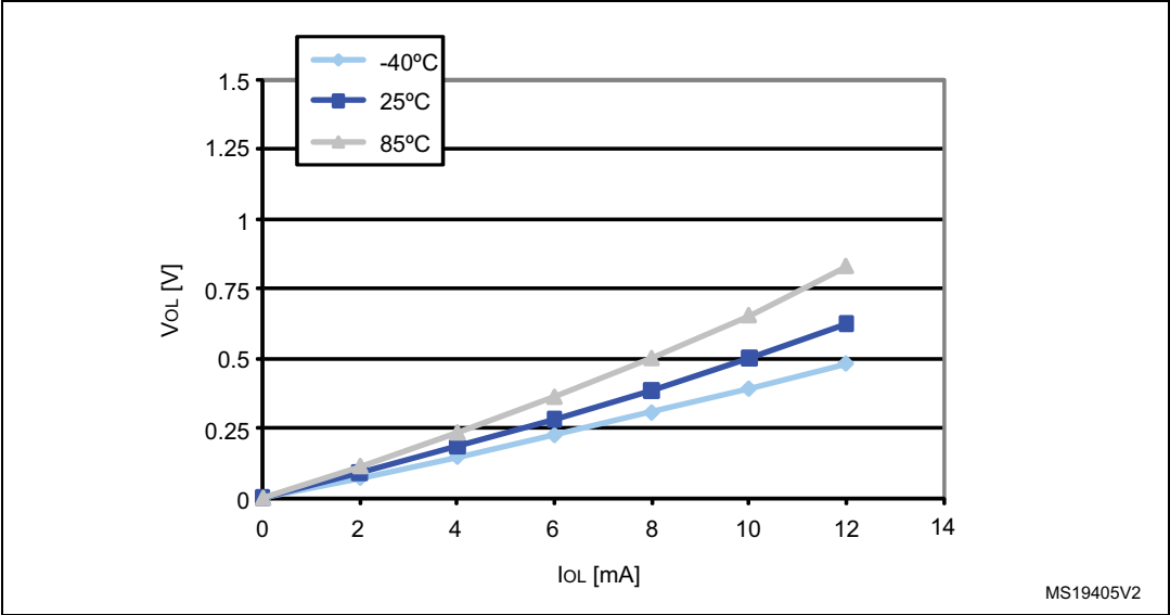
Figure 24. Typ. V_{OL} @ V_{DD} = 3.3 V (high sink ports)
