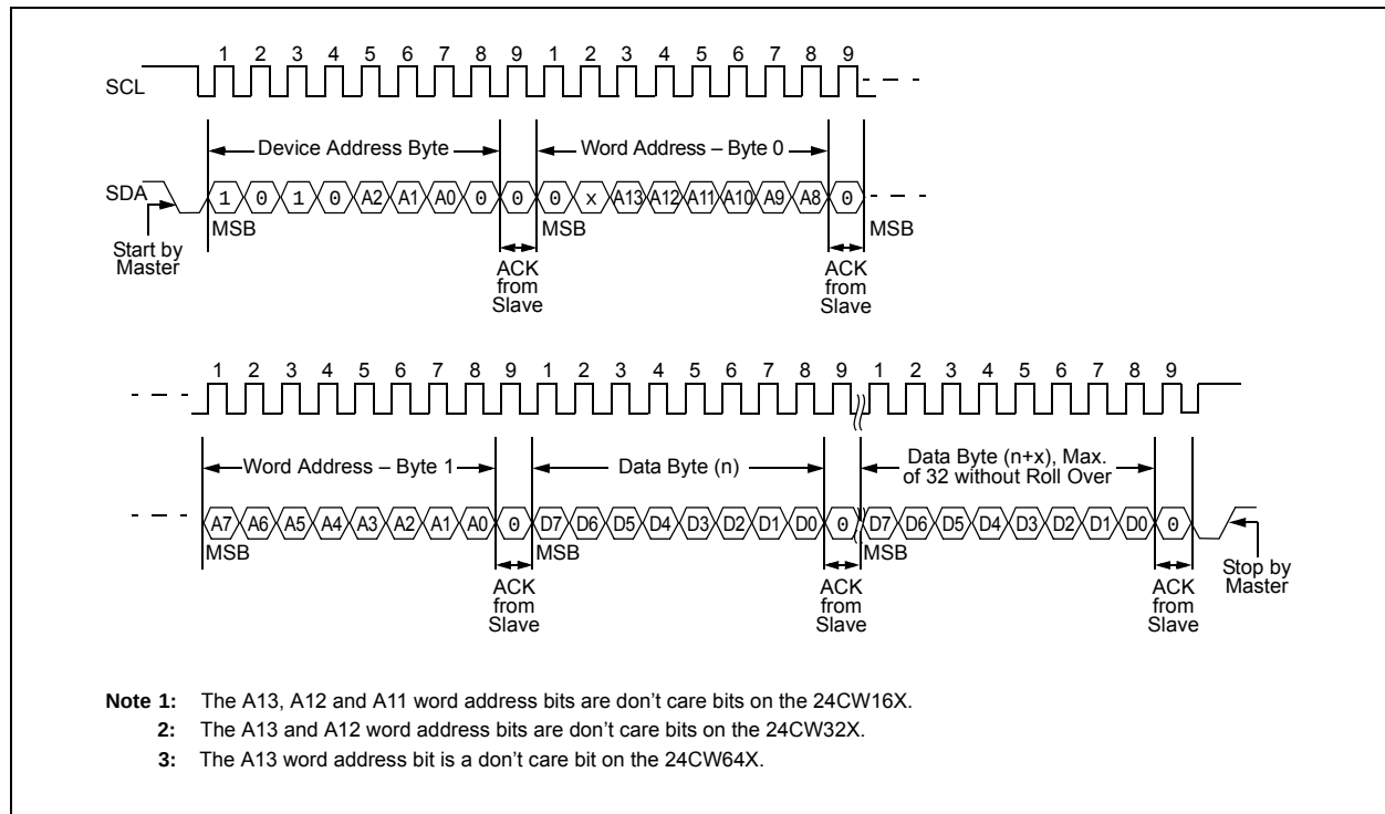
FIGURE 6-2: PAGE WRITE
