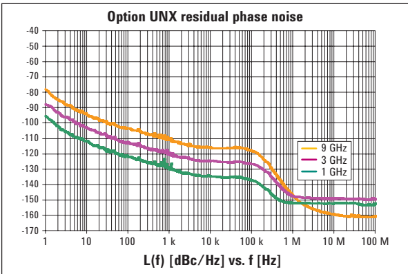
Measured phase noise (data collected with the E5500 and plotted without spurs)
