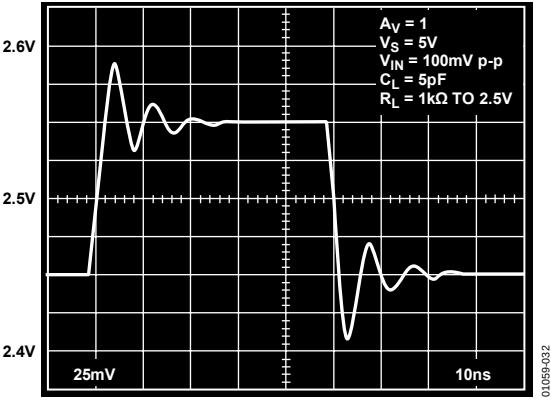
Figure 32. 100 mV Pulse Response, V_S = 5V
