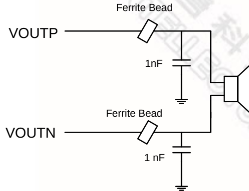
NAU82028 outputs connected to speaker with Ferrite Bead filter
