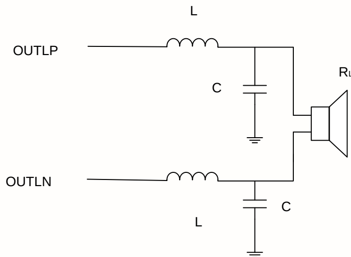
NAU82028 outputs connected to speaker with LC filter
