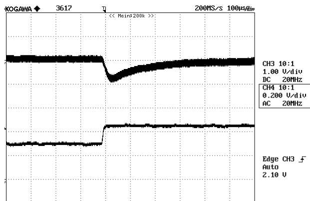
Figure 9: Output voltage response to step-change in load current (50%-75% of I_o , max; di/dt = 0.1A/\mu s ). Load cap: 10 \mu F tantalum capacitor and 1 \mu F ceramic capacitor. Top Trace: V_{out} (200mV/div, 100 \mu s /div), Bottom Trace: I_{out} (1A/div). Scope measurement should be made using a BNC cable (length shorter than 20 inches). Position the load between 51 mm to 76 mm (2 inches to 3 inches) from the module.
