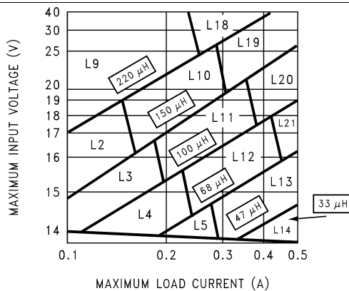
Figure 19. LM2671-12
