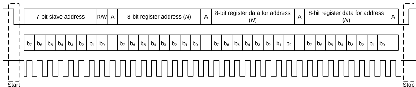
Figure 18. Typical I²C Sequence
