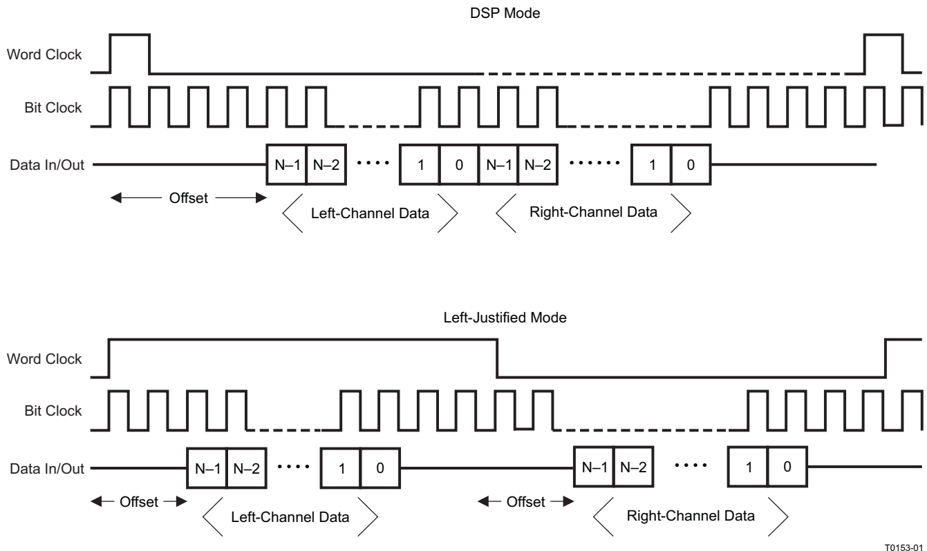
Figure 20. DSP Mode and Left-Justified Modes, Showing the Effect of a Programmed Data Word Offset
