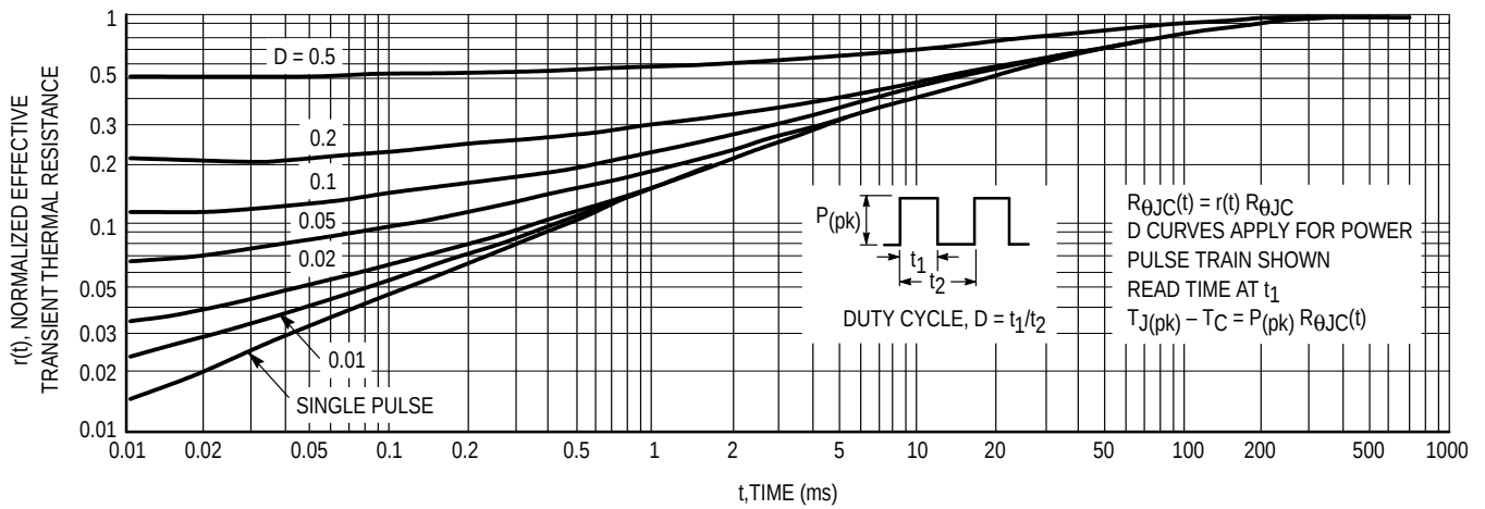
Figure 13. Thermal Response
