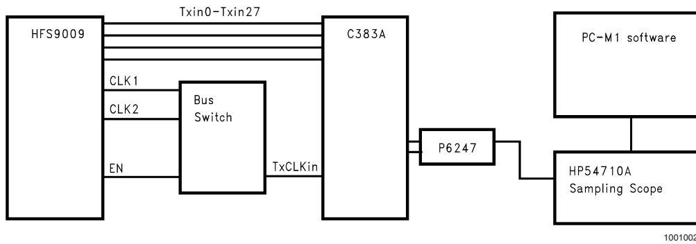
FIGURE 12. TJCC Test Setup
