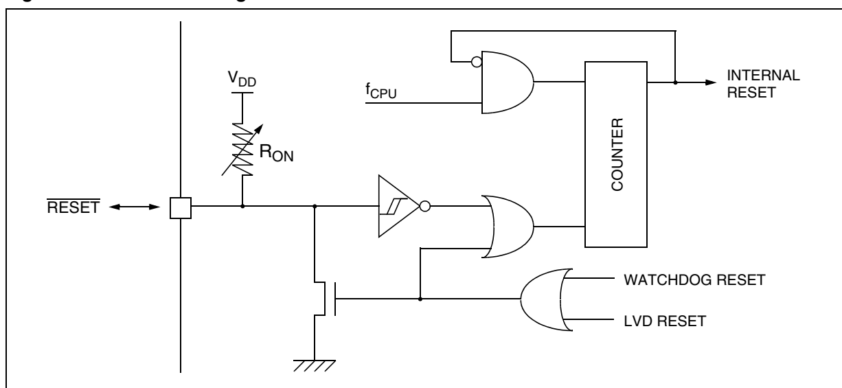
Figure 10. Reset Block Diagram
