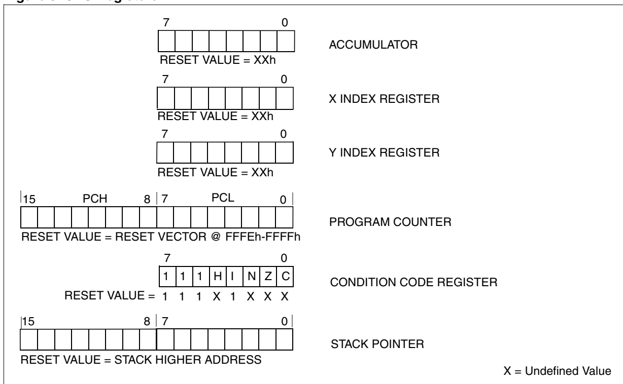
Figure 5. CPU Registers
