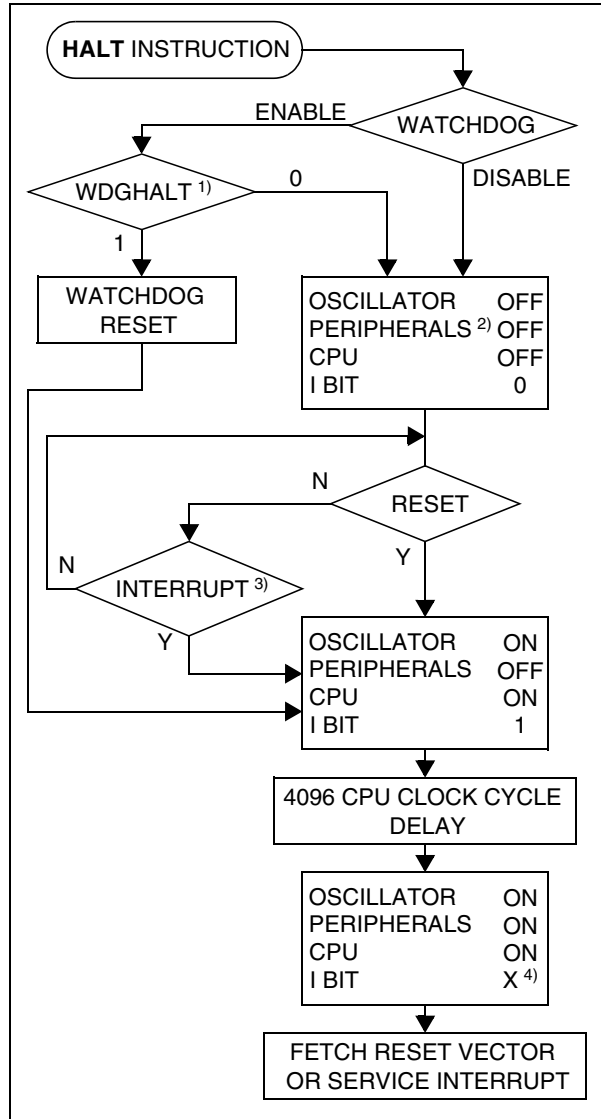
Figure 19. HALT Mode Flow-chart
