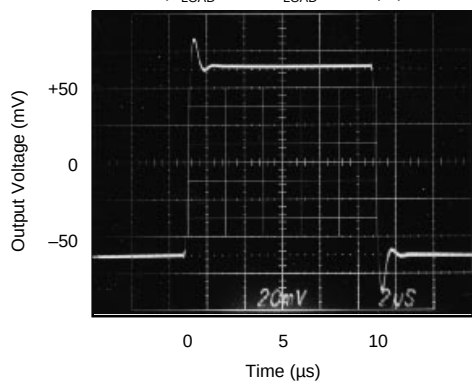
SMALL SIGNAL RESPONSE ( R_{\text{LOAD}} = \infty \Omega , C_{\text{LOAD}} = 1000\text{pF} )
