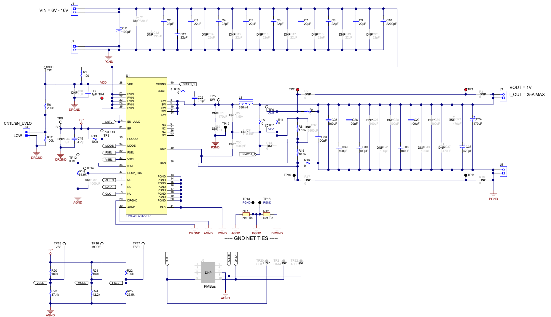
Figure 19. Typical Application Schematic
