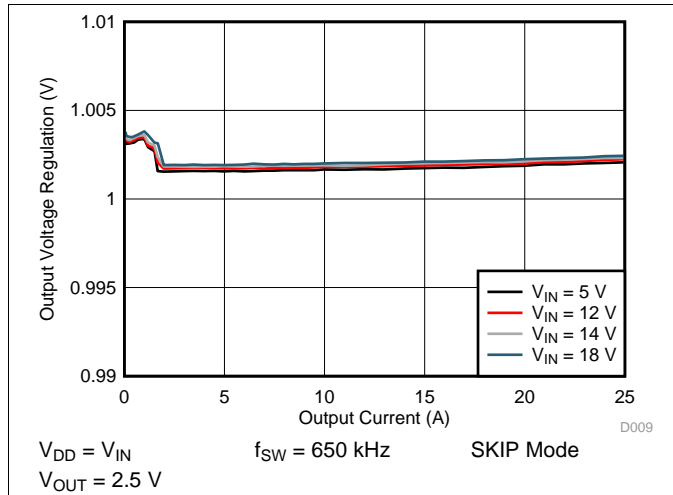
Figure 20. Output Voltage Regulation vs. Output Current
