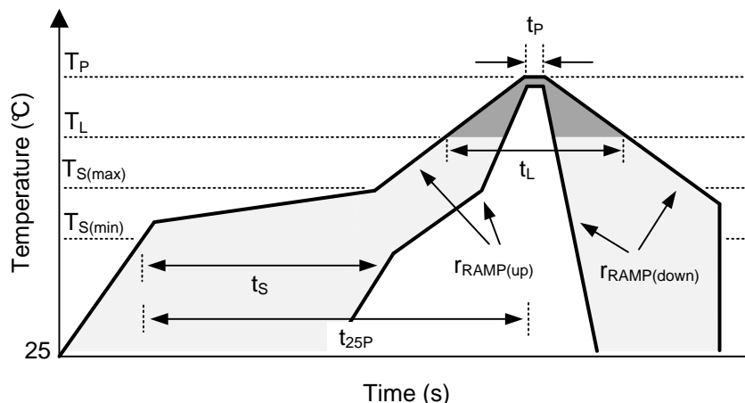
Figure 33. Recommended Reflow Oven Thermal Profile
