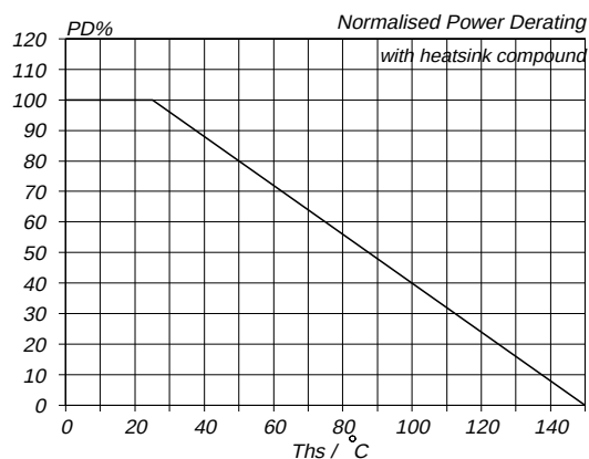
Fig. 10. Normalised power dissipation. PD\% = 100 \cdot P_D / P_{D 25^\circ C} = f(T_{mb})
