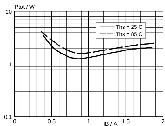
Fig. 8. Typical losses. P_{TOT} = f(I_B) ; I_C = 4 \text{ A} ; f = 16 \text{ kHz}
