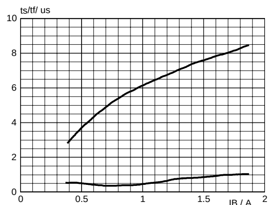
Fig. 9. Typical collector storage and fall time. ts = f(I_B) ; tf = f(I_B) ; I_C = 4.0 \text{ A} ; T_j = 85^\circ \text{C} ; f = 16 \text{ kHz}
