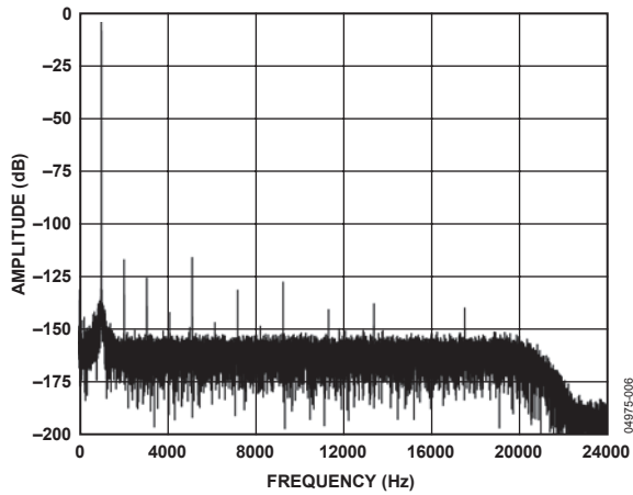
Figure 5. Normal Mode FFT, 1 kHz, -0.5 dB Input Tone, 256 \times Decimation
