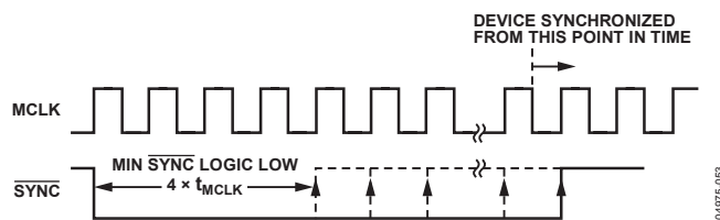
Figure 46. Recommended \overline{\text{SYNC}} Timing
