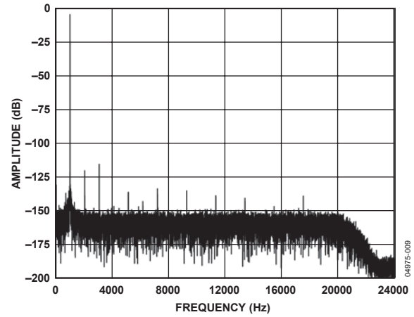
Figure 8. Low Power FFT, 1 kHz, -0.5 dB Input Tone, 256 \times Decimation
