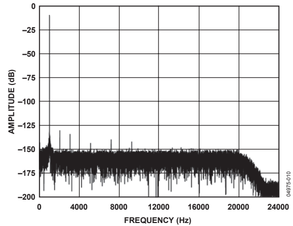
Figure 9. Low Power FFT, 1 kHz, -6 dB Input Tone, 256 \times Decimation
