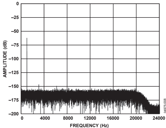
Figure 7. Normal Mode FFT, 1 kHz, -60 dB Input Tone, 256 \times Decimation
