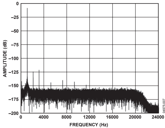
Figure 6. Normal Mode FFT, 1 kHz, -6 dB Input Tone, 256 \times Decimation
