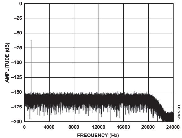
Figure 10. Low Power FFT, 1 kHz, -60 dB Input Tone, 256 \times Decimation
