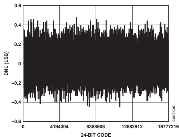
Figure 35. 24-Bit DNL
