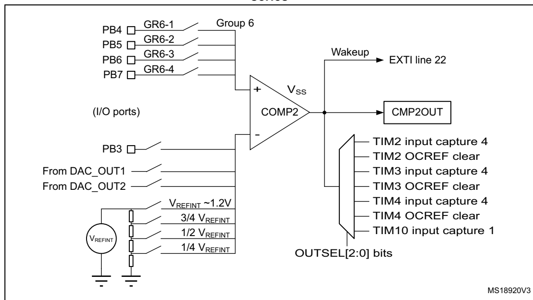
Figure 6. COMP2 interconnections (Cat.3, Cat.4, Cat.5 and Cat.6 devices), STM32L1 series
