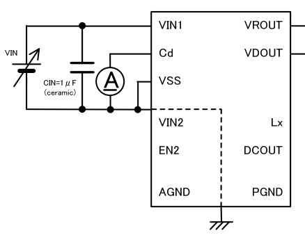
Circuit No.6
