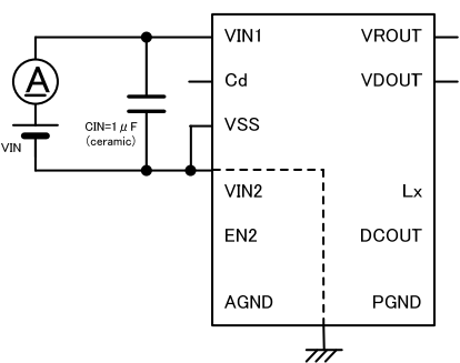
Circuit No.2
