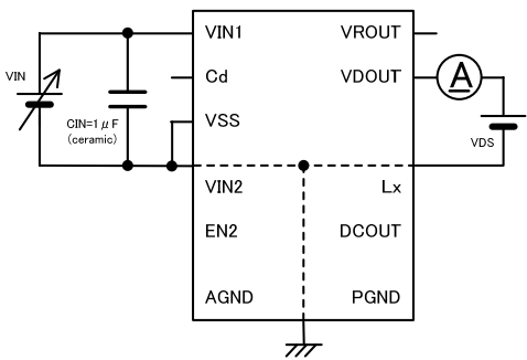
Circuit No.5
