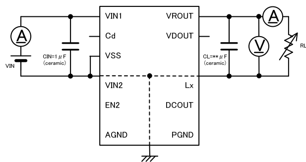
Circuit No.3
