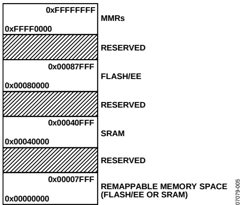
Figure 10. Memory Map
