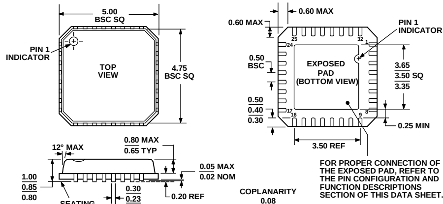
Figure 30. 32-Lead Lead Frame Chip Scale Package [LFCSP_VQ] 5 mm × 5 mm Body, Very Thin Quad (CP-32-4)
