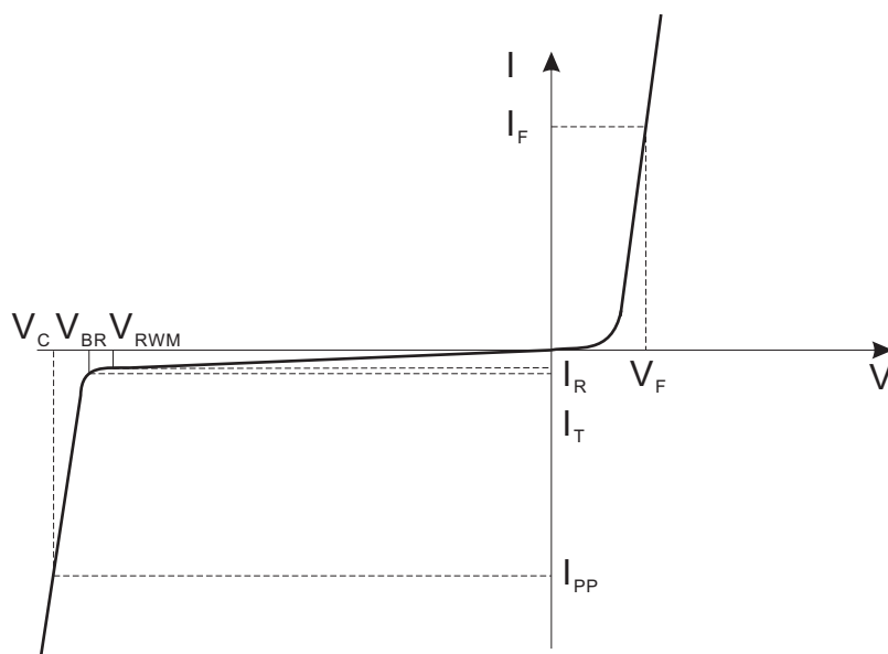
Uni-Directional TVS
