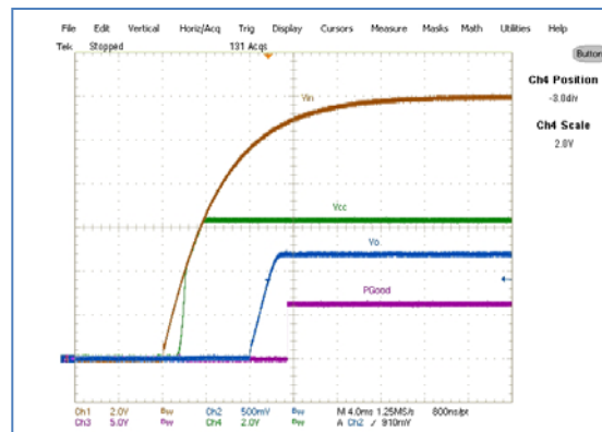
Figure 33: Start up at 4A Load, Ch1: V_{in} , Ch2: V_o , Ch3: PGGood, Ch4: Vcc
