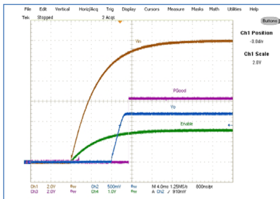
Figure 32: Start up at 4A Load, Ch1: V_{in} , Ch2: V_o , Ch3: PGGood, Ch4: Enable
