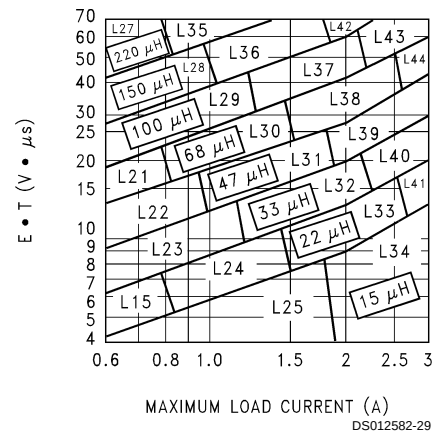
FIGURE 7. LM2599-ADJ
