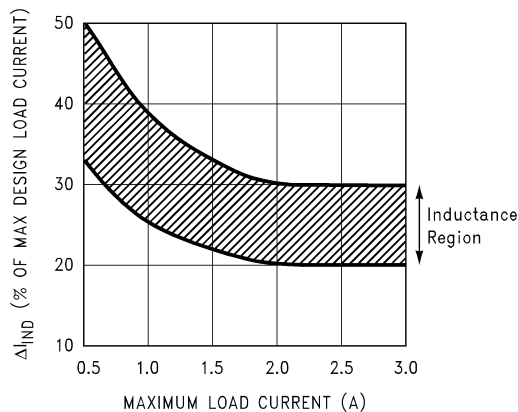
FIGURE 18. ( \Delta I_{LIND} ) Peak-to-Peak Inductor Ripple Current (as a Percentage of the Load Current) vs Load Current
