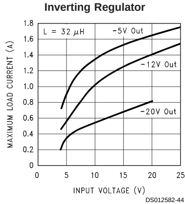
FIGURE 27. Maximum Load Current for Inverting Regulator Circuit
