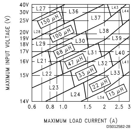
FIGURE 6. LM2599-12
