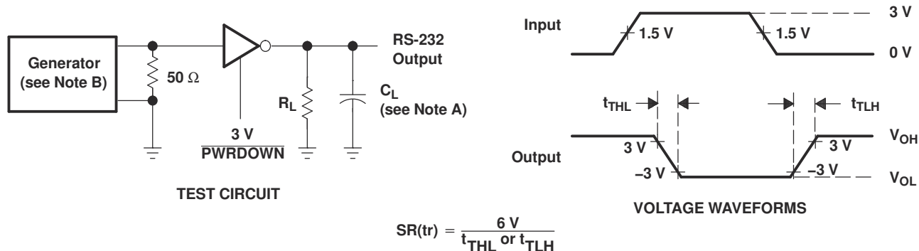
图 7-1. Driver Slew Rate
