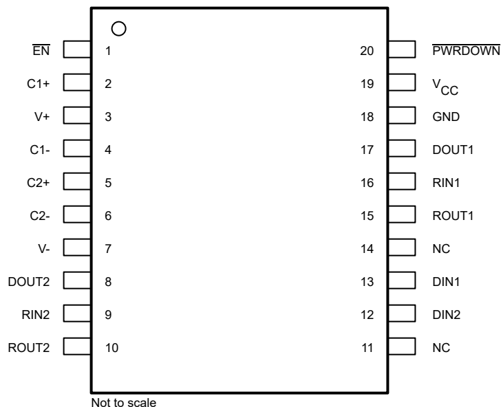
图 5-1. DB, DW, or PW Package (Top View)
