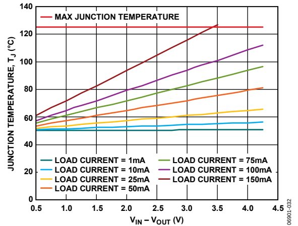
Figure 38. TSOT, 100 mm² of PCB Copper, T_A = 50^\circ\text{C}
