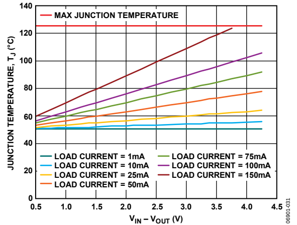
Figure 37. TSOT, 500 mm² of PCB Copper, T_A = 50^\circ\text{C}
