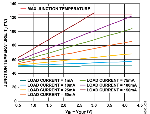
Figure 39. TSOT, 0 mm² of PCB Copper, T_A = 50^\circ\text{C}
