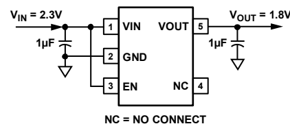
Figure 1. ADP121 TSOT with Fixed Output Voltage, 1.8 V
