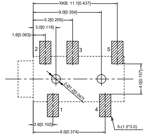
PCB LAYOUT TOP VIEW TOLERANCES: ±0.05
