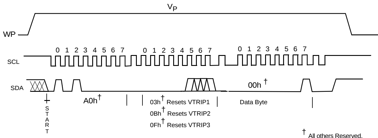
Figure 23. Resetting the V_{TRIPx} Level
