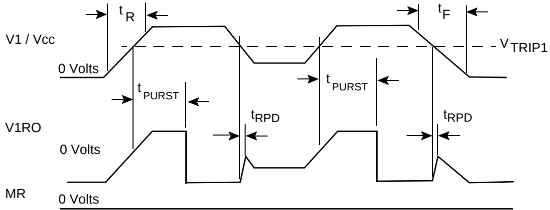
Figure 30. Power-Up and Power-Down Timing
