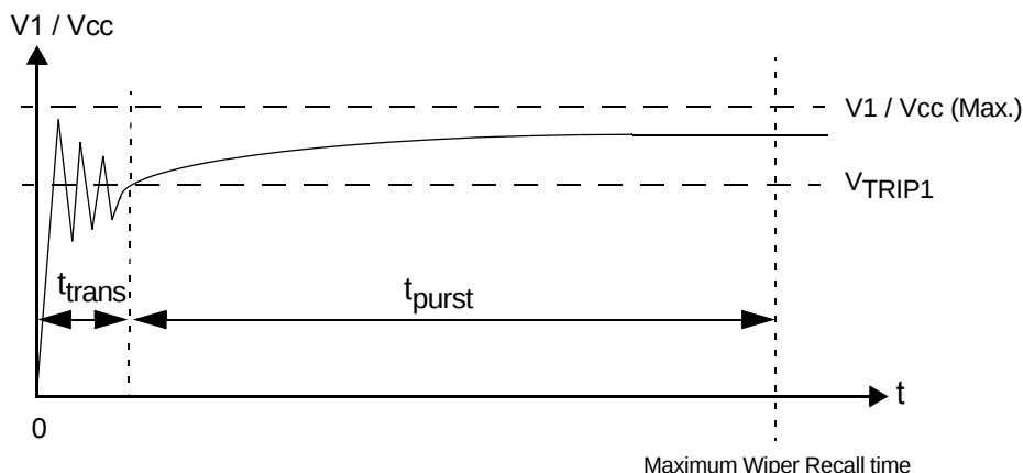
Figure 7. DCP Power
