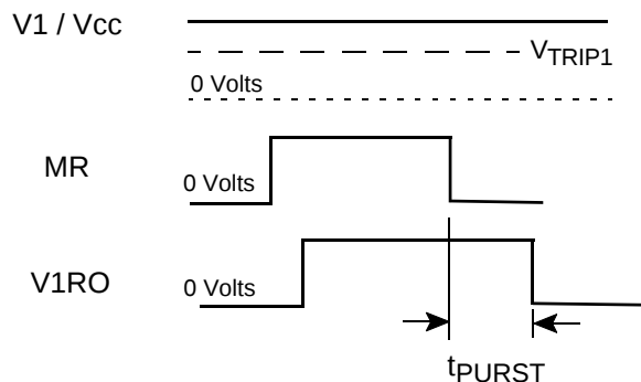
Figure 20. Manual Reset Response
