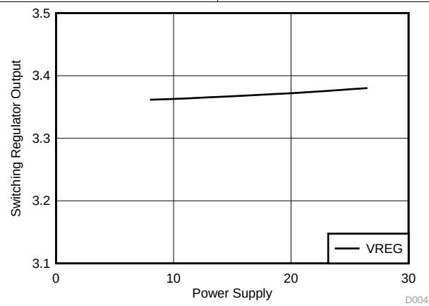
Figure 2. Switching Regulator Output vs Power Supply (VregSel = 0)
