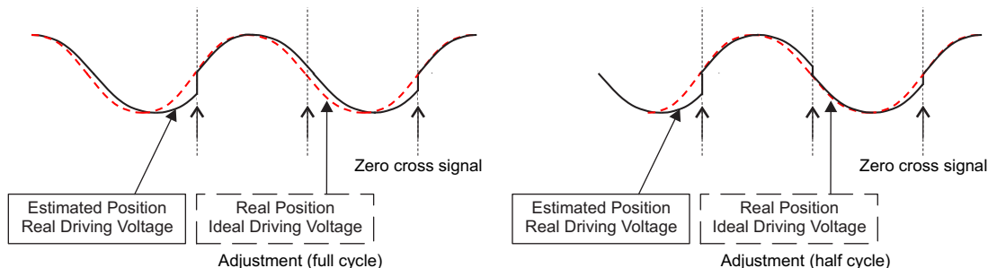
Figure 20. Closed Loop Control Commutation Adjustment Mode
