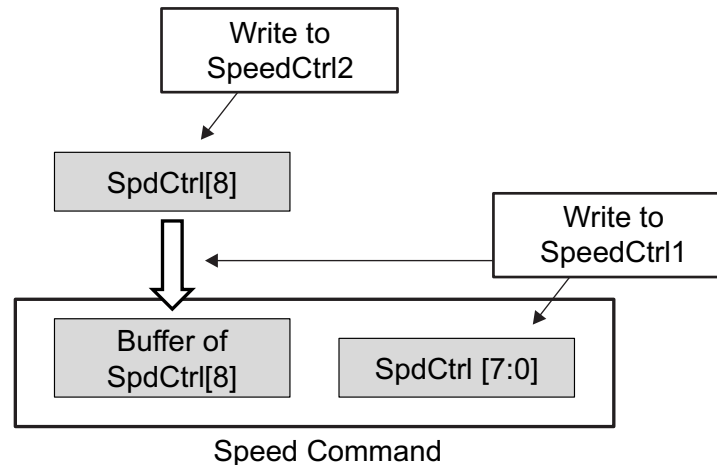
Figure 23. I²C Mode Speed Control
