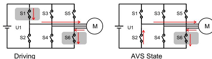
Figure 35. Inductive AVS
