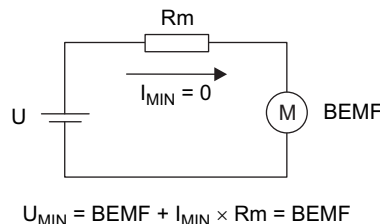
Figure 33. Mechanical AVS
