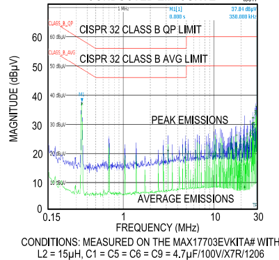
4.2V OUTPUT, 10A CHARGING CURRENT CONDUCTED EMI CURVE
