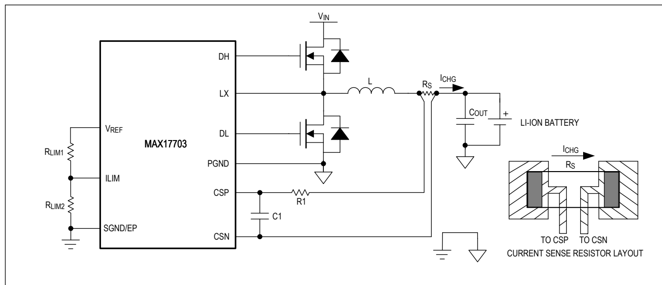
Figure 5. Current-Sense Circuit
