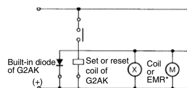
Set or reset coil
