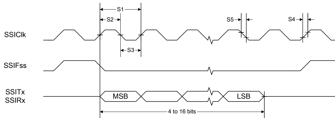
图 22-20. SSI Timing for TI Frame Format (FRF=01), Single Transfer Timing Measurement
