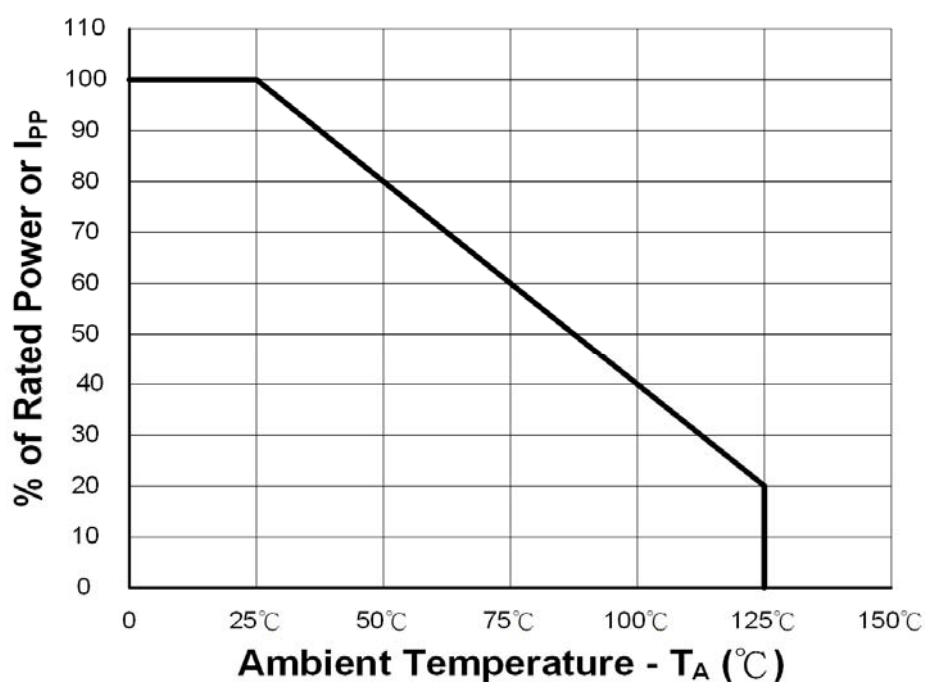
Figure 1. Power Detating
