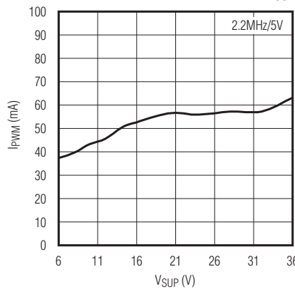
PWM MODE SUPPLY CURRENT vs. V_{SUP}
