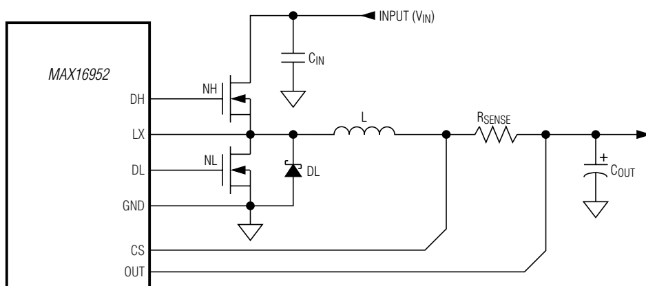
a) OUTPUT SERIES RESISTOR SENSING
