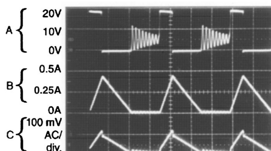
Discontinuous Mode Switching Waveforms
