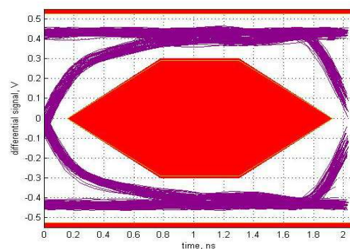
Figure 43. High-Speed Downstream Port 2
