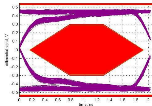
Figure 39. Downstream Port 3
