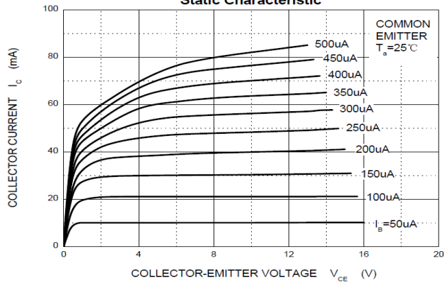
Static Characteristic
