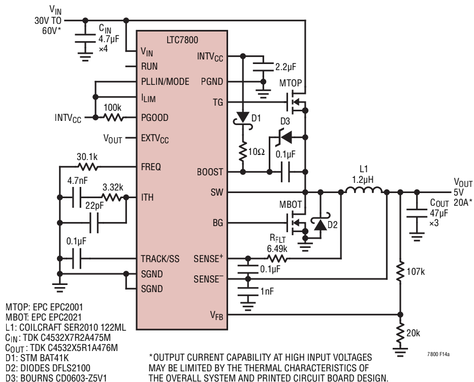
Figure 14. High Efficiency 5V 450kHz Step-Down Regulator Using GaN FETs
