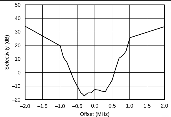
Figure 4-9. Typical Selectivity at 250 kBaud Data Rate, 868 MHz, GFSK, IF is 304 kHz and the Digital Channel Filter Bandwidth is 540 kHz
