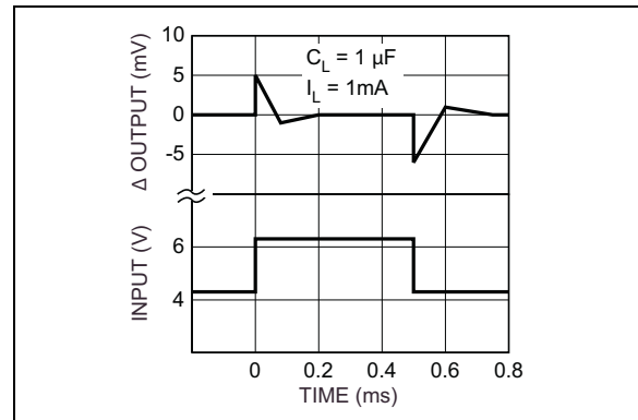
FIGURE 2-17: Line Transient.
